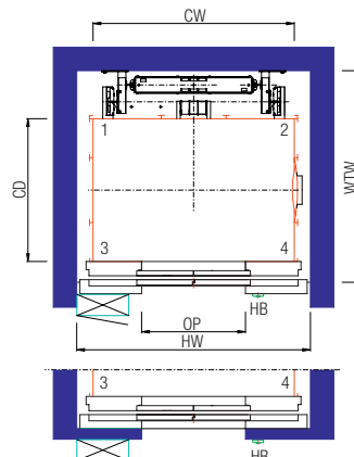
1 entrance
