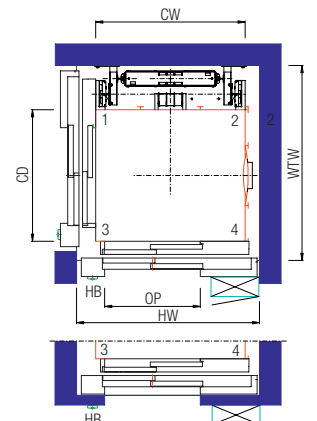
2 entrances (90°)
