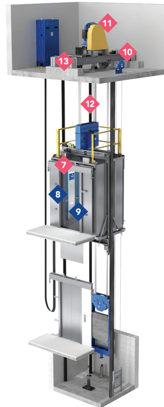
Arise MOD Plus 2:1 arrangement, AC Gearless machine example.
