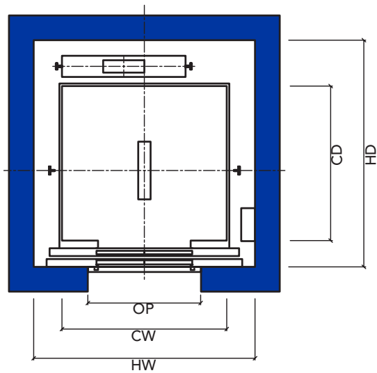
Hoistway Plan
