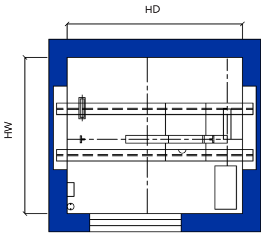
Typical Machine Room Plan
